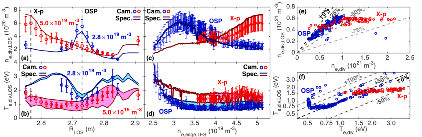
Fig. 4. Example radial profiles of line-integrated n_{e,div} (a) and T_{e,div} (b) at the onset of detachment (blue) and in deep detachment (red) show agreement primarily within 20% between the spectroscopic measurements and synthetically derived line integrals of the 2D estimates. Similar agreement is observed throughout the n_e ramp for both n_{e,div} (c) and T_{e,div} (d) at the outer strike point (blue) and above the X-point (red). The solid lines in (a–d) correspond to the spectroscopic measurements (Spec.), whereas the line integrals of the 2D estimates inferred from the camera analysis (Cam.) are plotted with data points. The shaded regions in (b, d) cover the bracket between the upper and lower limits of the T_e measurements. The line-integrated measurements underestimate n_{e,div} (e) by 25–40% at the outer strike point (blue) and by up to 75% at the X-point (red). For T_{e,div} (f), the line integral provides a good representation of the local T_{e,div} at the outer strike point (blue) with the exception of the T_{e,div} \approx 0.5 \text{ eV} range, while underestimation by up to 50% is observed at the X-point (red). The black dashed lines indicate similarity between the line-integrated and local values ( n_{e,div,LOS}/n_{e,div} = n_{e,div,LOS}/n_{e,div} ) in both (e) and (f), and the grey dashed lines correspond to underestimation of the local n_{e,div} by 25%, 50% and 75% in (e) and under- and/or overestimation of the local T_{e,div} by 50% and 100% in (f). Note the logarithmic axes in (f).
