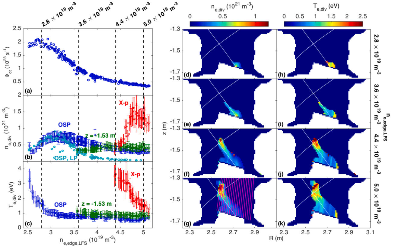
Fig. 3. Detachment of the outer divertor during the n_e ramp is indicated by roll-over and decay of the total ion current at the outer divertor target (a). The estimated 2D n_{e,div} distributions (d–g) and local values (b) show peaking of n_{e,div} at the outer strike point (OSP, blue) after the onset of detachment in agreement with the Langmuir probe data (LP, cyan), as well as steep increase of n_{e,div} above the X-point (X-p, red) at the highest n_{e,edge,LFS} and only subtle increase halfway between the aforementioned locations ( z = -1.53 \text{ m} , green). The 2D T_{e,div} estimates (h–k) and the local values (c) suggest decrease of T_{e,div} from 3–4 eV to 0.5 eV at the outer strike point and to 1.0–1.5 eV above the X-point with almost constant temperature at around 1.0 eV halfway between the outer strike point and the X-point. The vertical black dashed lines in (a–c) indicate the upstream densities presented in (d–k). The spectroscopic lines-of-sight used for line-integrated analysis are visualized with magenta lines in (g).
