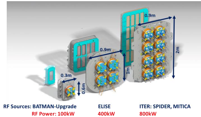
FIG. 10: The RF sources development in a step-ladder approach towards ITER with the support of the EUROfusion facilities BATMAN Upgrade and ELISE [from ref. 63].
