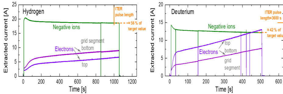
FIG. 11: ELISE time traces of the extracted negative ion current and co-extracted electron current measured separately for the top and bottom segment of the extraction system during long pulses with the new CW High-Voltage power supply in hydrogen (left) and deuterium (right). [From Ref. 12]
