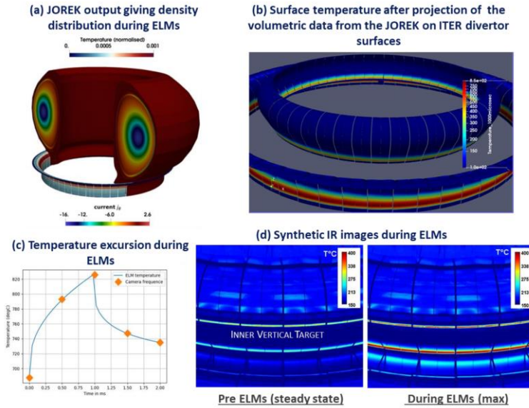
FIG. 4: ITER simulation of transient ELMs in the IR synthetic diagnostic: (a) density distribution computed from JOREK, (b) volumetric data from the JOREK projected onto first-wall divertor surfaces, (c) temperature evolution, (d) synthetic images during ITER ELMs [from 9].
