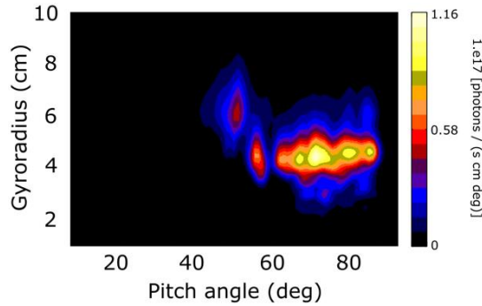
FIG. 7: Simulated FILD measurements of the velocity-space distribution (as a function of gyroradius and pitch angle) of the escaping ions for ITER baseline scenario obtained with the synthetic diagnostic FIELDSIM combined with an ASCOT simulation for calculating the fast ion losses at the diagnostic location.
