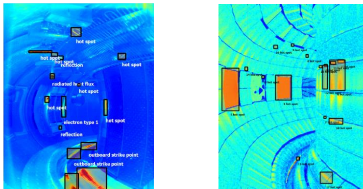
FIG. 5: (left) WEST wide-angle IR images and automatic thermal events detection [from ref. 37]. (right) ITER simulated IR image where thermal events are automatically detected using algorithm trained on WEST data.
