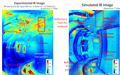
FIG. 3: WEST experimental (left) and simulated (right) IR images calculated with the synthetic diagnostic [from ref. 28].
