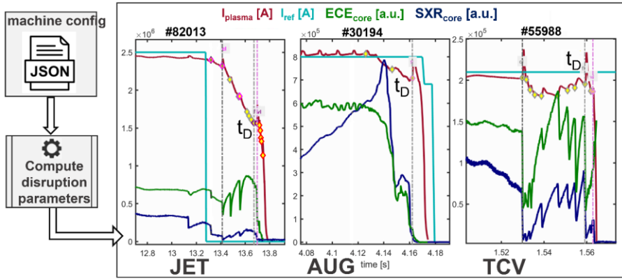
FIG. 9: Automatic calculation of disruption characteristic times based on the correlation of various quantities, where I_{\text{plasma}} is the plasma current, I_{\text{ref}} is the reference plasma current, ECE_{\text{core}} and SXR_{\text{core}} are proxies for the core temperature based respectively on Electron Cyclotron Emission and on Soft X-rays. [from Ref. 11]
