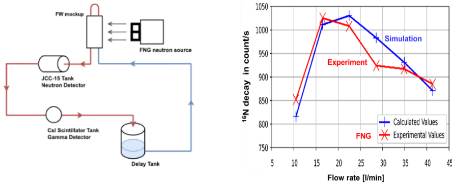
FIG. 17: (left) Water activation experimental set-up at FNG with the neutron (Inventory Sample Neutron Coincidence Counter model JCC-15) and gamma CsI detectors and water expansion tank to increase the count rates [from 77]; (right) ^{16}\text{N} decay in FNG water activation experiment: experimental & simulated ^{16}\text{N} decay counts with FLUNED versus flow rate when the neutron source was positioned at a distance of 5cm from the component [from 98].
