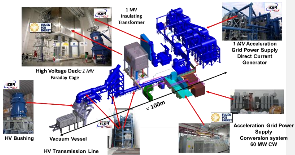
FIG. 13: Overview of the MITICA power supply system [from ref. 14]. The components in blue are provided by the Japanese domestic agency.
