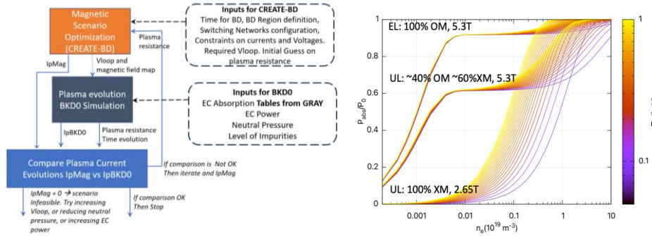
FIG. 2: (left) General layout of the CREATE-BD/BKD0/GRAY coupling scheme for breakdown simulations; (right) ITER simulation: EC absorption for O-mode (OM) injection from EL and UL at 5.3 T and X-mode (XM) injection from UL at 2.65 T [from ref. 6].
